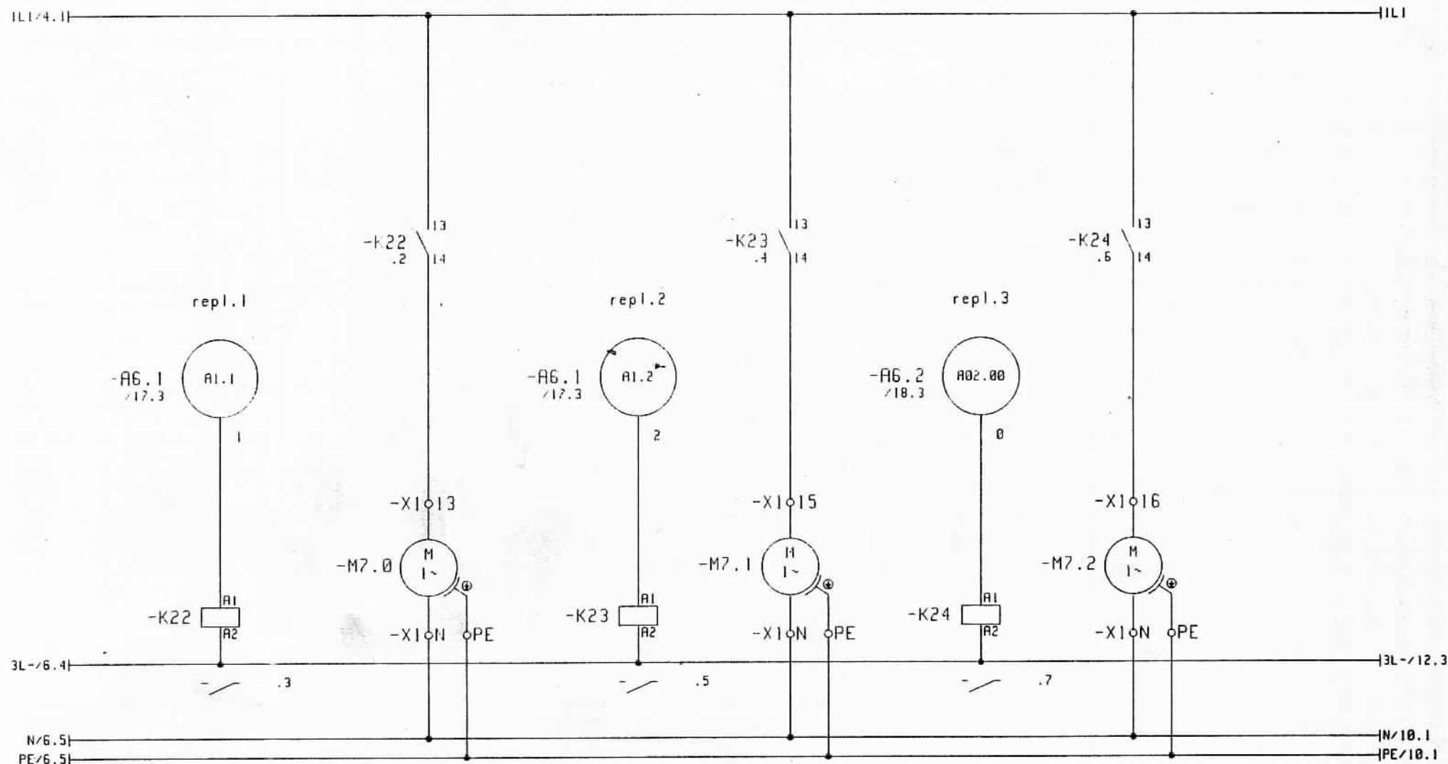
Regenerierung Tank 3 replanishment tank 3
